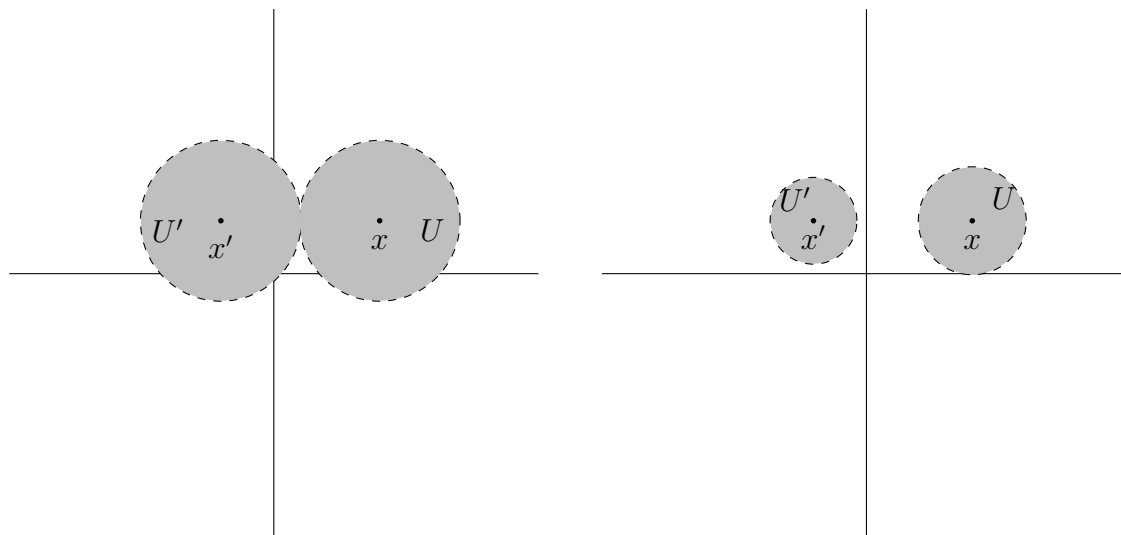
Figure 15.1: On the left, two open sets U and U' “separating” x from x' . On the right, another possible choice for U and U' (for the same x and x' as on the left).
